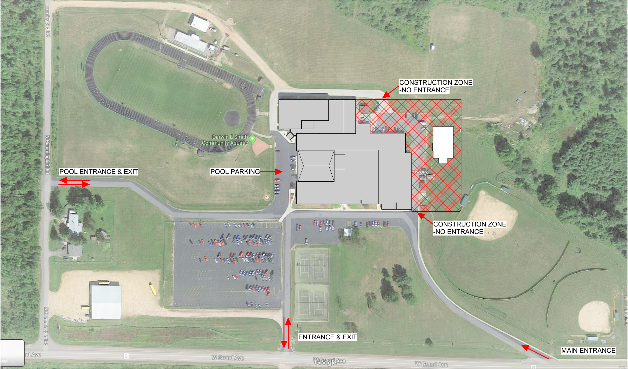
1 WITTENBERG-BIRNAMWOOD HIGH SCHOOL CONSTRUCTION SITE TRAFFIC PLAN SCALE 1" = 160'-0"
